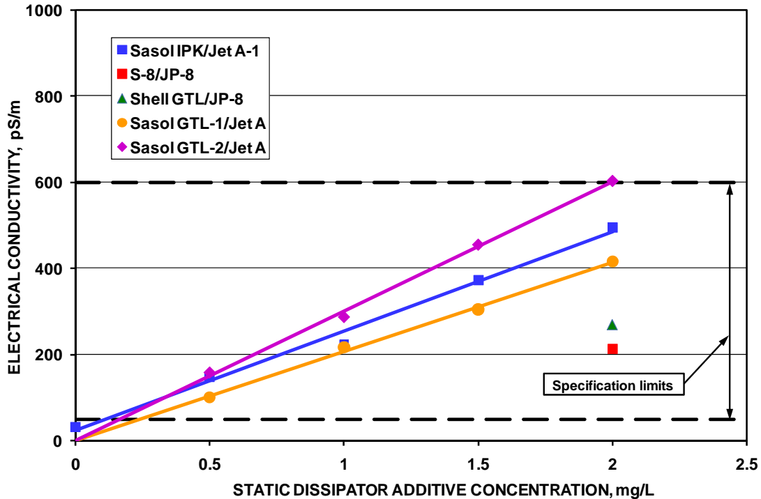
Figure 13. Response of SSJF to Static Dissipator Additive
